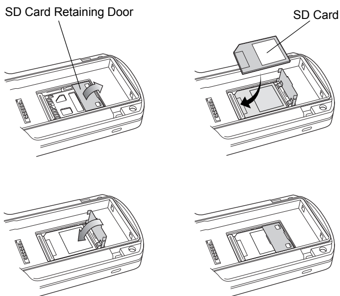
Figure 4-7 Inserting the SD Card
